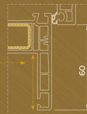
IDEAL NEO MD RENOVERINGSRAMME 40 mm
